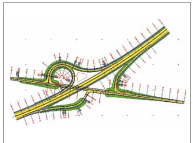
Crearea planurilor vizuale atractive de inalta performanta si functionalitate . (Detalii intersectie, Departement of Infrastructure, Lausanne, CH)
